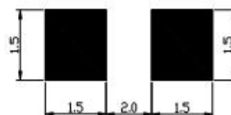
● Paecommended Soldering Pattern
